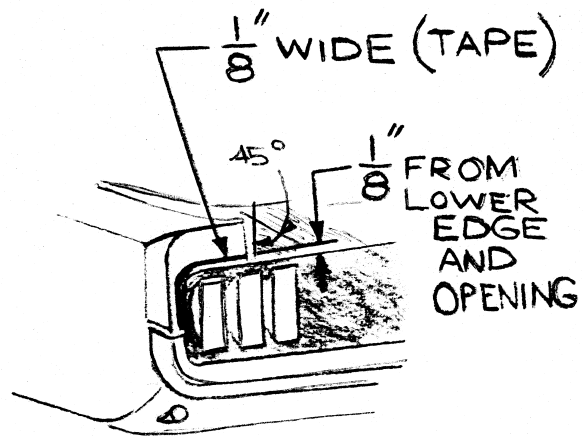
DETAIL - REAR (1969 BOSS 302 ONLY)
